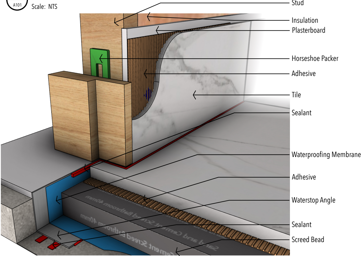
3 Unenclosed Shower Waterstop - Detail A101 Scale: NTS
