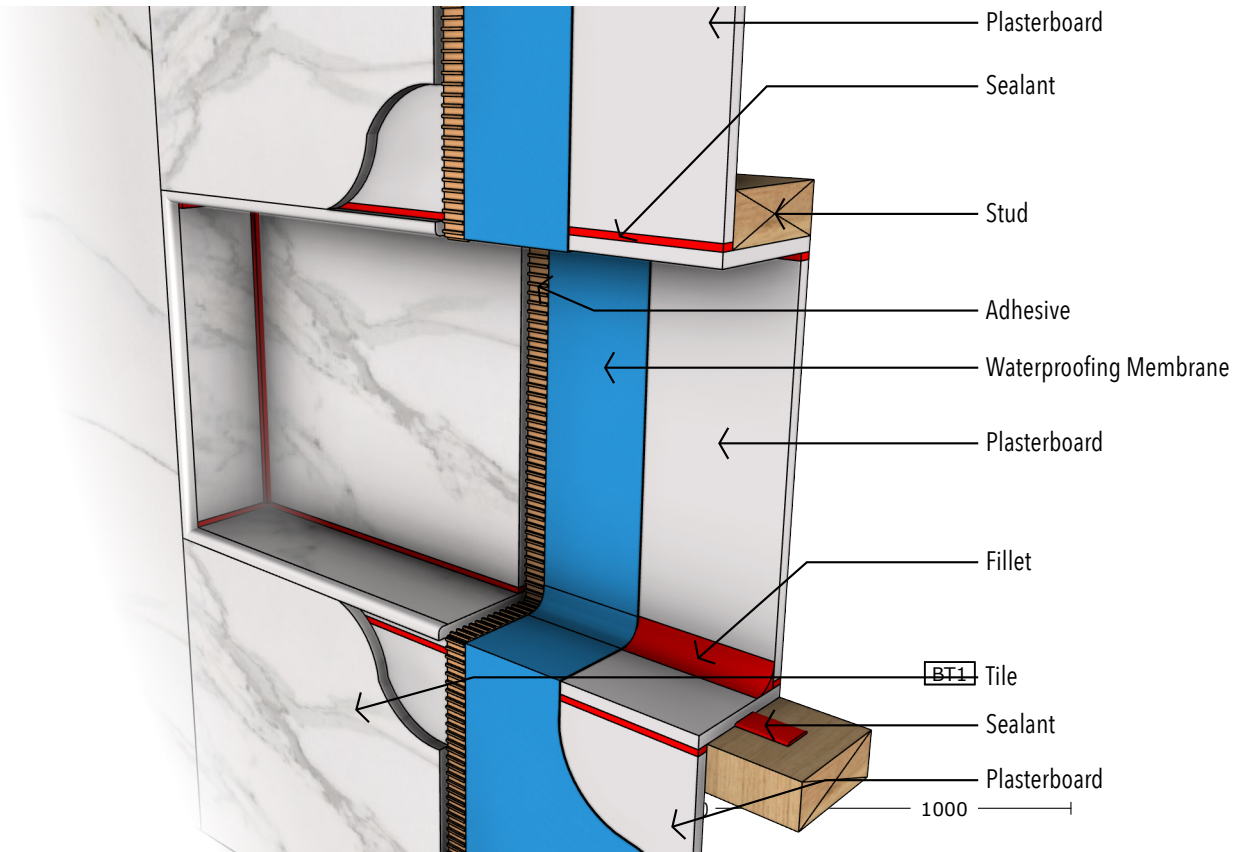
4 Shower Penetration & Niche- Detail A101 Scale: NTS
